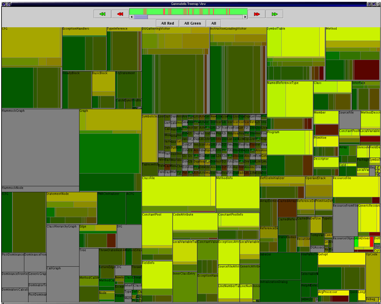
Figure 8: JABA execution data visualized in GAMMATELLA.
