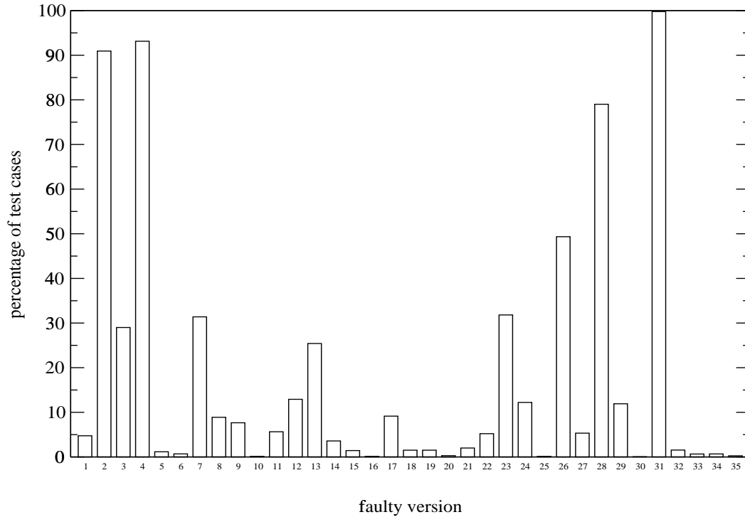
Figure 14: Bar chart that shows the percentages of inputs in the test pool for Space that expose faults in the versions of the program.
