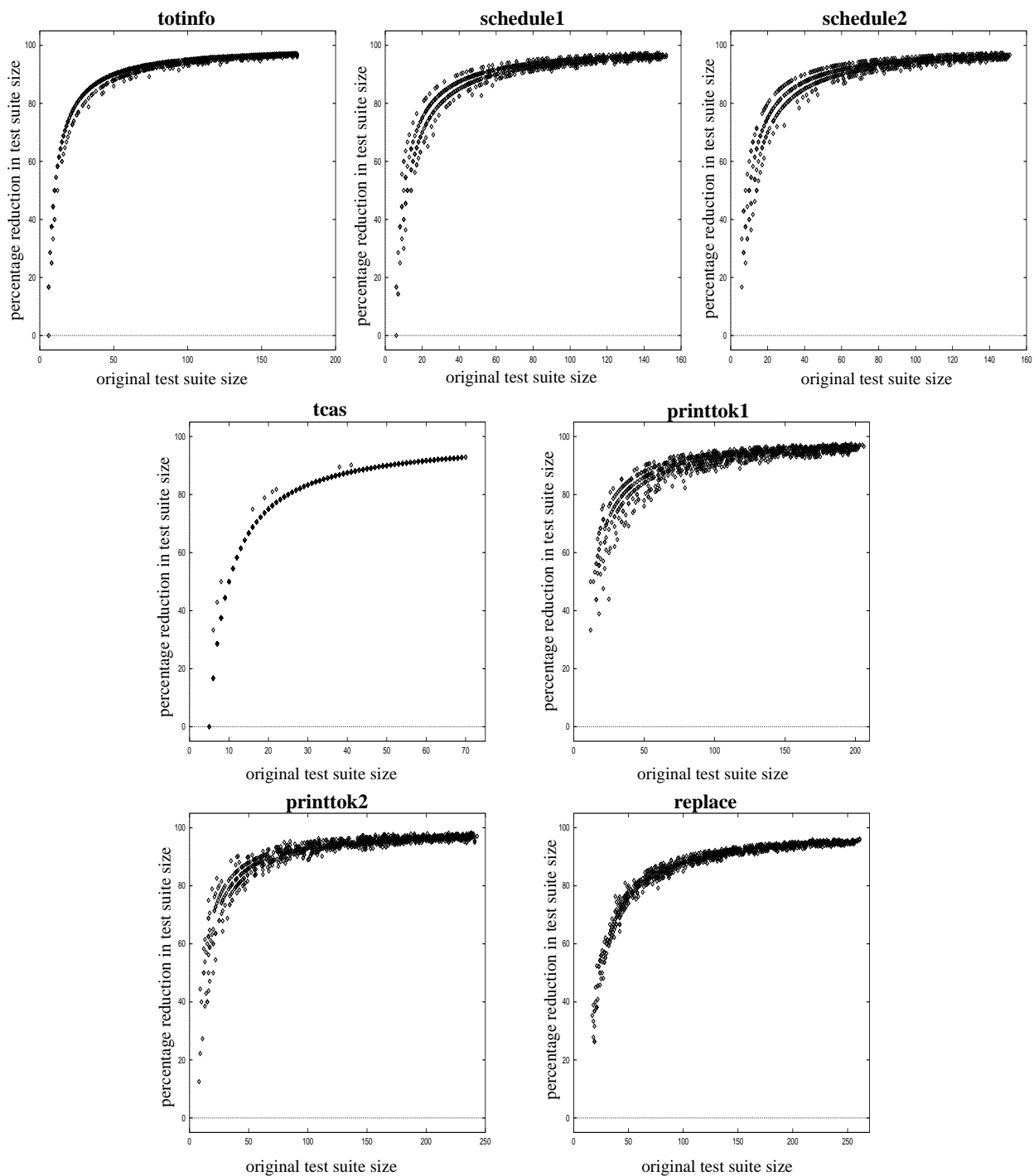
Figure 4: Percentage reduction in test-suite size as a result of test-suite reduction versus sizes of original test suites, for edge-coverage-adequate test suites. Horizontal axes denote sizes of original test suites, and vertical axes denote percentage reductions in test-suite size.
