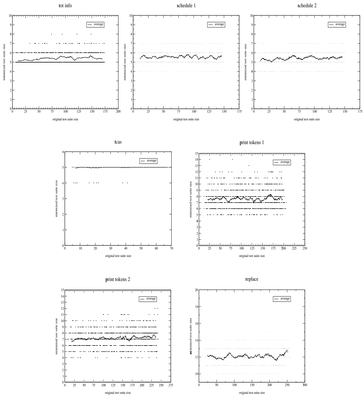
Figure 3: Sizes of test suites reduced for edge coverage versus sizes of original test suites, for edge-coverage-adequate test suites. Horizontal axes denote sizes of original test suites, and vertical axes denote sizes of reduced test suites. Average reduced test-suite size across the range of original test-suite sizes (computed as running averages over each set of fifty consecutive points) is denoted by the solid lines.
